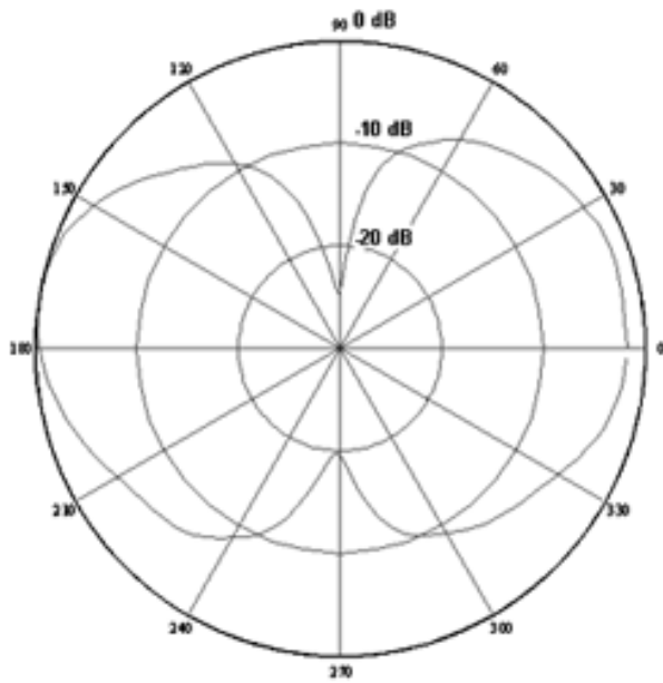
Radiation Pattern (H-Plane)
