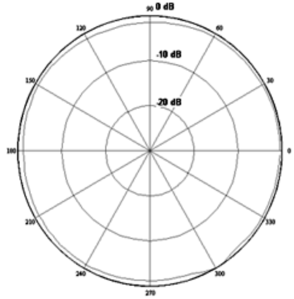
Radiation Pattern (E-Plane)
